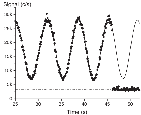
FIG. 3: Interference fringes : number of atoms detected per second as a function of time (counting period : 0.1 s). The position x_{M3} of mirror M_3 is swept as a function of time. We have verified that the fringe period corresponds to a displacement \Delta x_{M3} = \lambda_r/2 = 335 \text{ nm} . The background signal of the detector, measured by flagging the lithium beam 50 s later, is shown on the right part of the figure and its average value 3370 counts/s is represented by the dot-dashed line. The data points are fitted by a sine curve, whose argument is the sum of linear and a quadratic functions of time (this last term being needed to represent the piezo hysteresis). From this fit, we extract the value of the fringe contrast equal to 74% with an error of the order of 1%.
